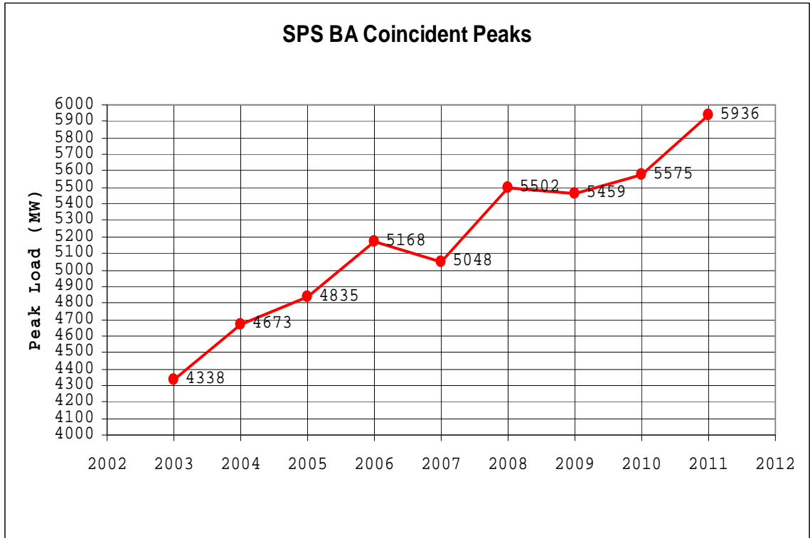
Figure 7 SPS BA Coincident Peaks
