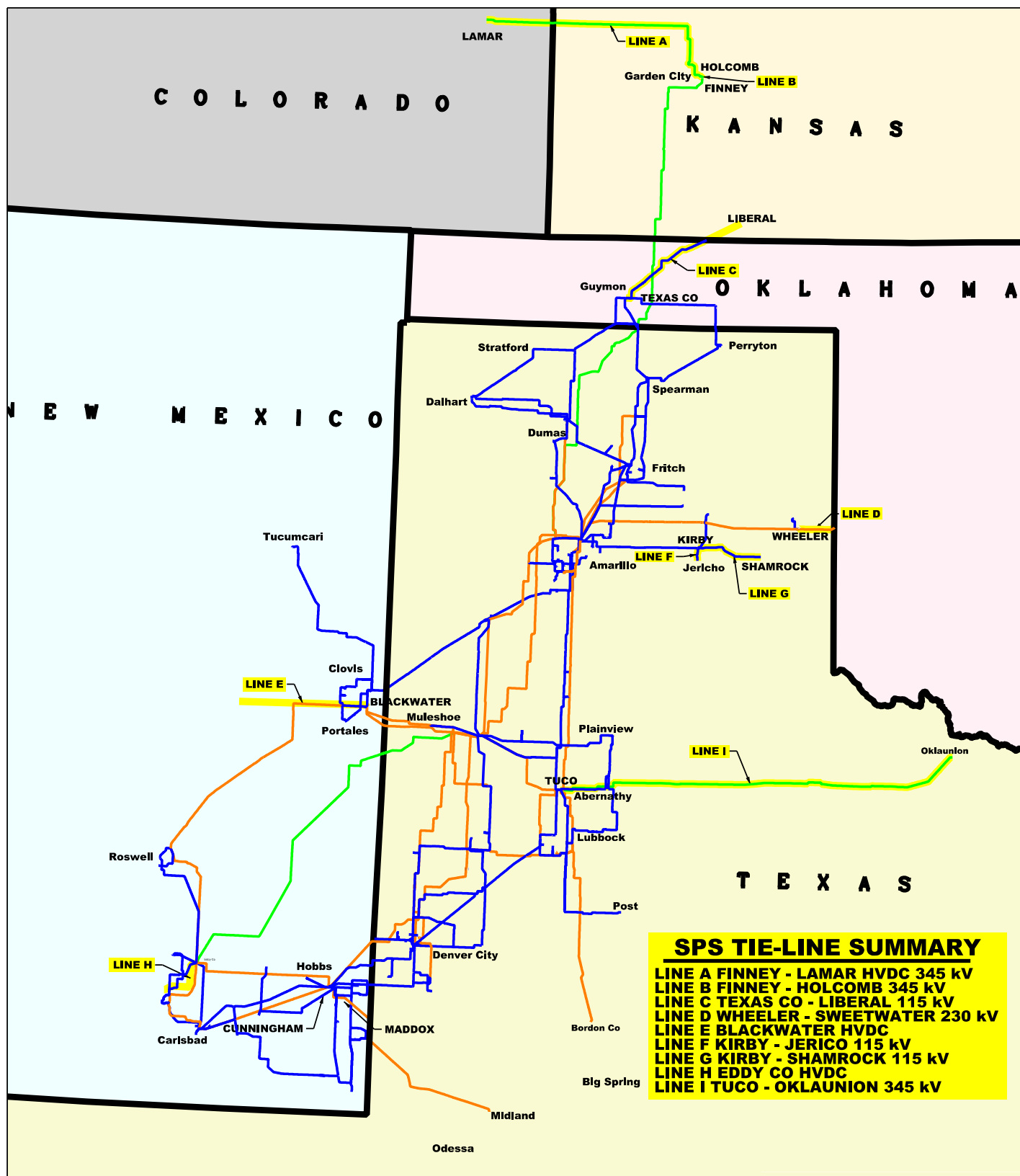
Figure 2 – SPS Transmission Interconnections
